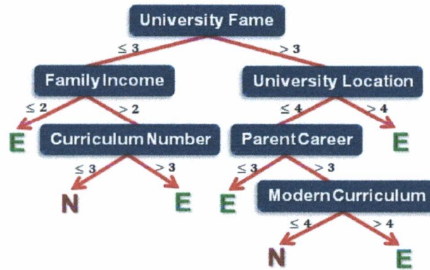
Figure 3 Generated visualization of decision tree.
