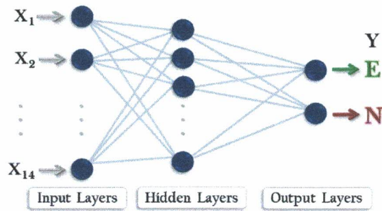
Figure 2 ANN network used for data classification
