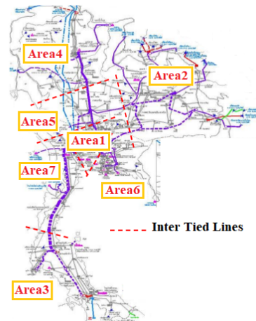
Fig. 1. Overview of a modified Thailand power system base case in 2019.
