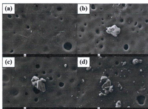
Figure 3. FE-SEM image of separators of (a) PSF (b) PSF with 0.5% \text{CaTiO}_3 , (c) PSF with 1.0% \text{CaTiO}_3 and (d) PSF with 2.0% \text{CaTiO}_3 .
