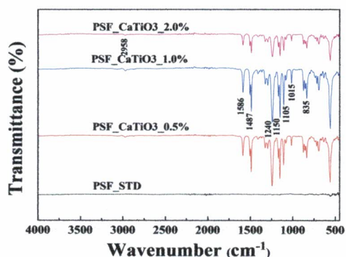
Figure 4. FT-IR spectra of \text{CaTiO}_3 -filled PSF separators.
