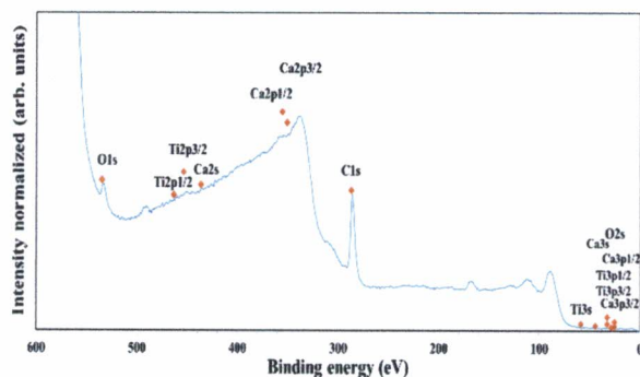
Figure 5. XPS spectra of supercapacitors with 2 wt% \text{CaTiO}_3 -filled polysulfone separators.
