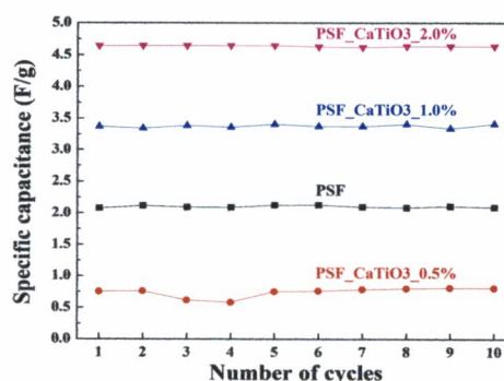
Figure 6. Specific capacitance of supercapacitors with \text{CaTiO}_3 -filled polysulfone separators.
