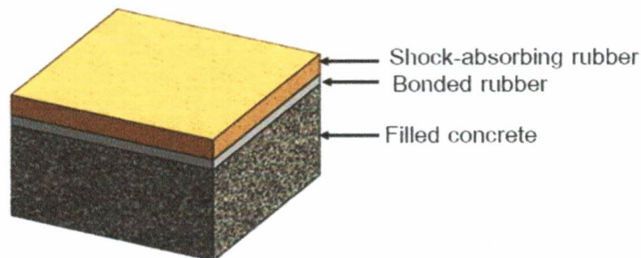
Figure 1 Dimension and components of paving blocks
