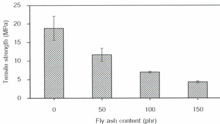
Figure 8 Tensile strength of bonded rubber
