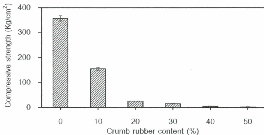
Figure 6 Compressive strength of concrete mixed with crumb rubber
