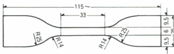
Figure 4 Dumbbell-shaped Die-C specimen
