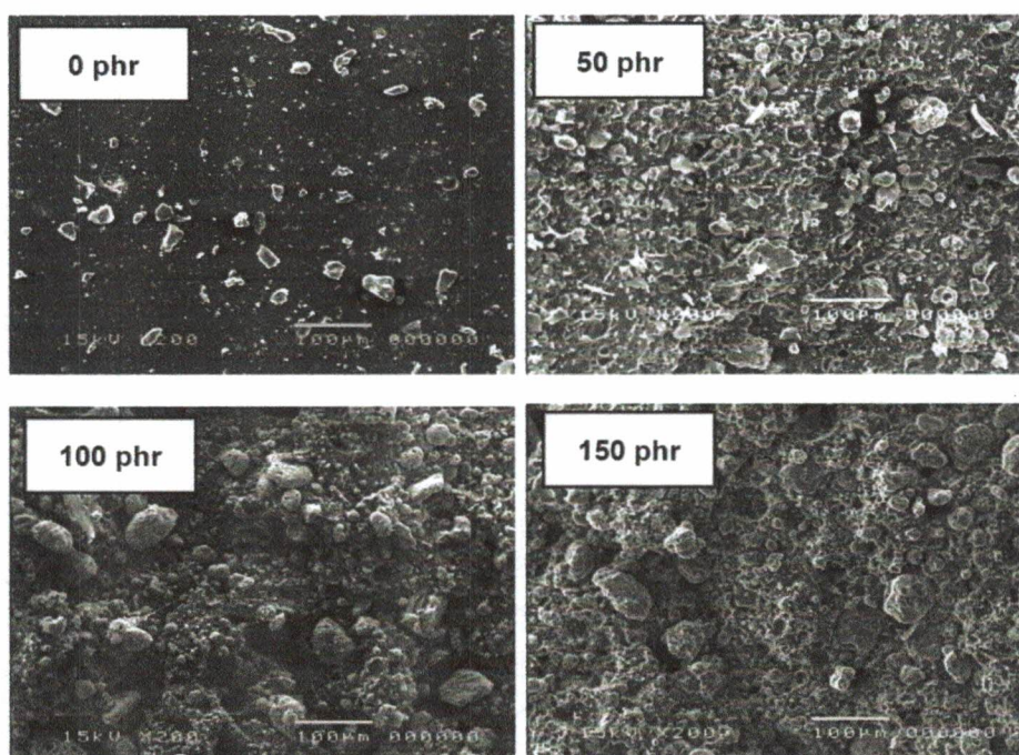
Figure 10 The morphology of fracture surface of bonded rubber prepared from natural rubber with modified fly ash content
