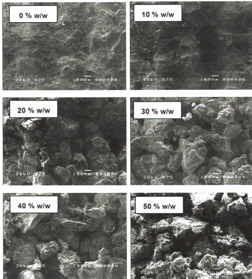
Figure 7 Morphology of concrete mixed with crumb rubber
