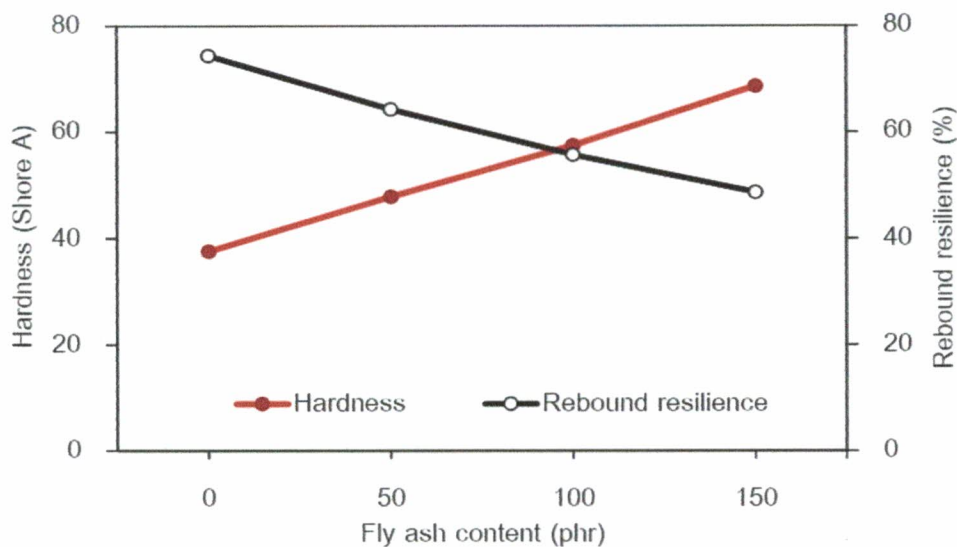
Figure 11 Hardness and rebound resilience of bonded rubber
