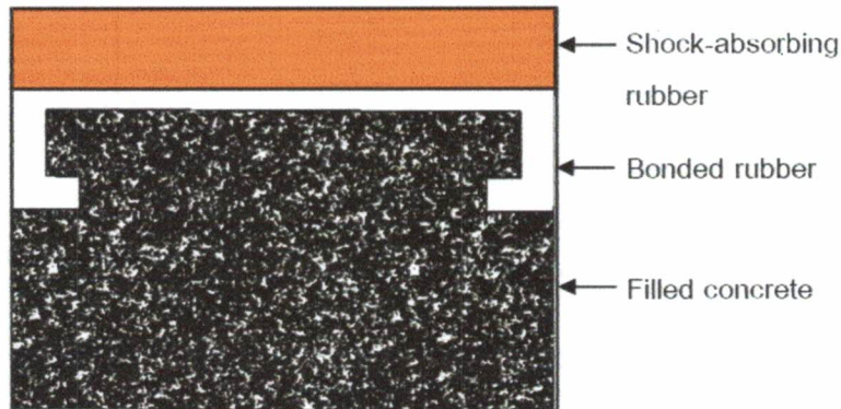
Figure 13 Cross-sectional image of a paving block
