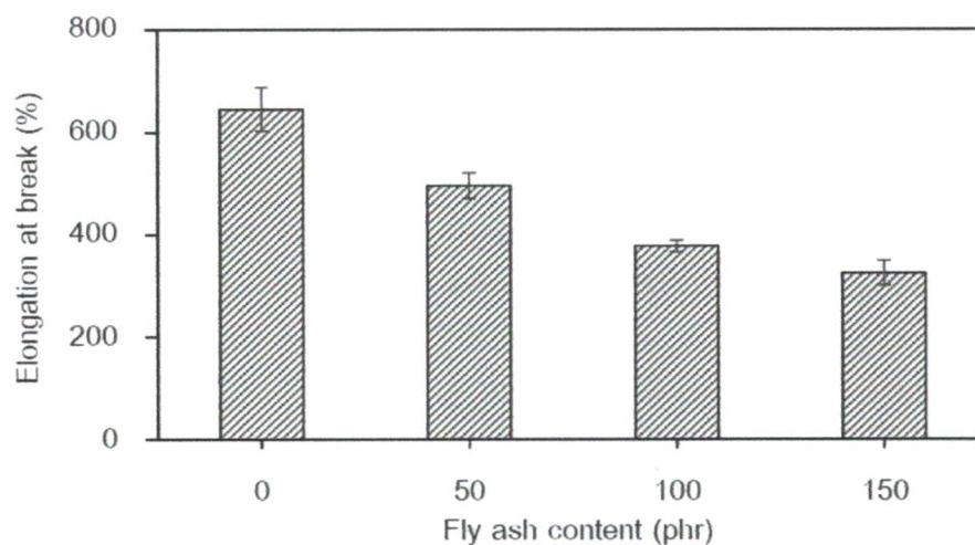
Figure 9 Elongation at break of bonded rubber
