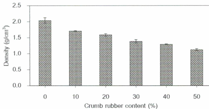
Figure 5 Density of concrete mixed with crumb rubber
