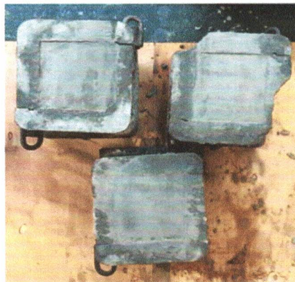
Figure 3 Concrete cubic mold sized 10x10x10 centimeters
