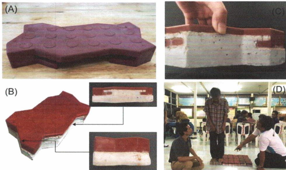
Figure 14 (A) Shock-absorbing rubber [1] (B) Paving blocks (C) Pulling adhesion test (D) Paving blocks test
