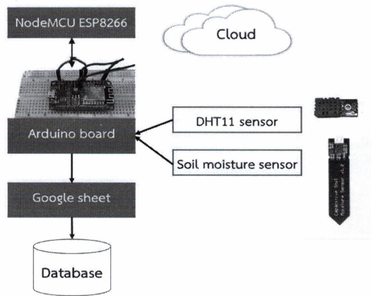
Figure 2 Process flow of IOT system for planting maize.
