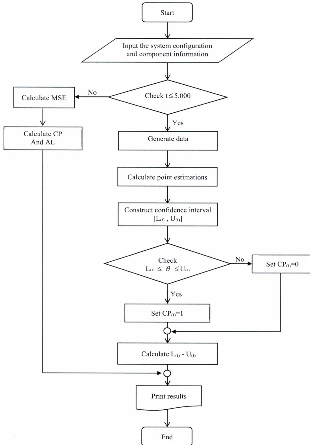
Figure 1. Monte Carlo simulation flowchart.
