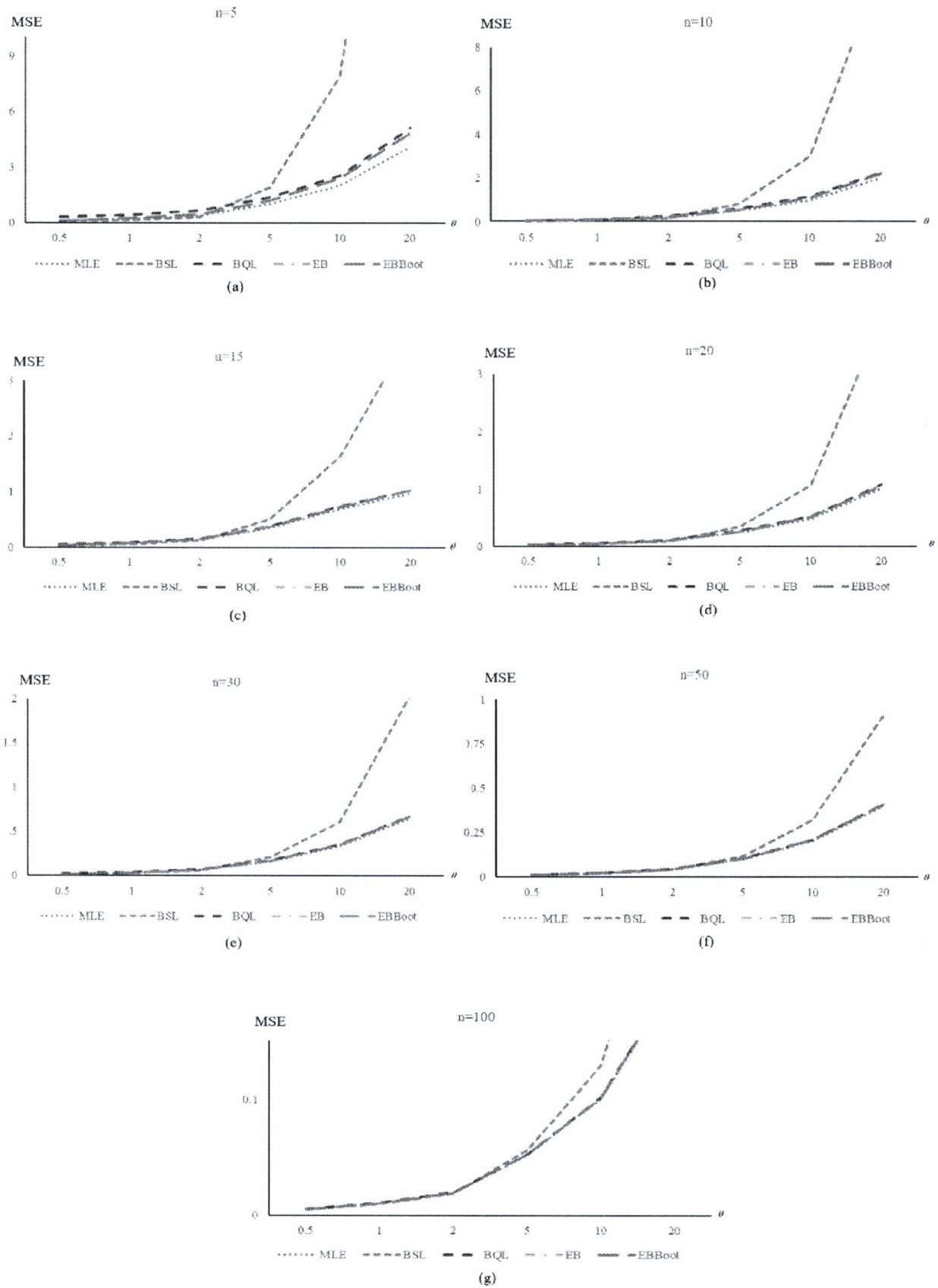
Figure 2. Comparative performance of point estimation.
