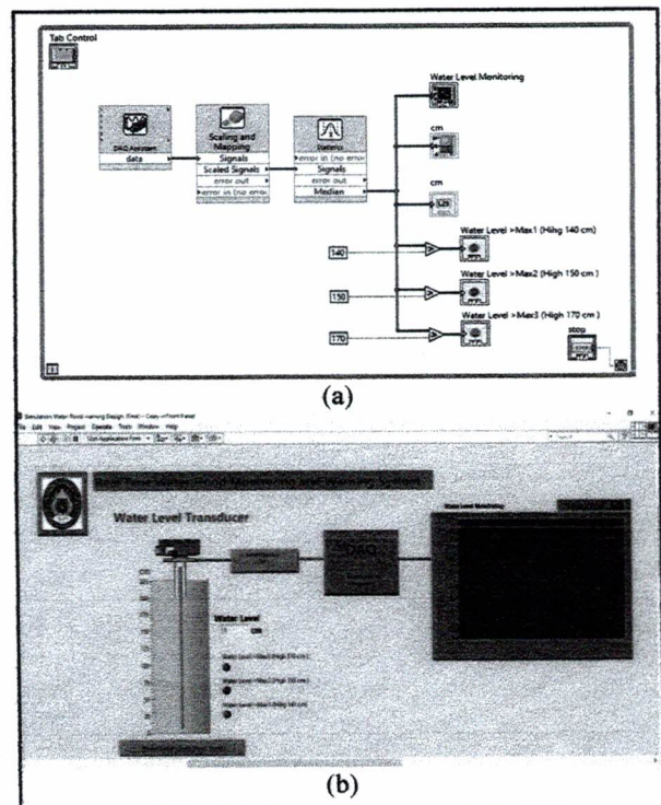
Fig. 6 Measurement program (a) and water level monitoring screen on LabVIEW program (b).
