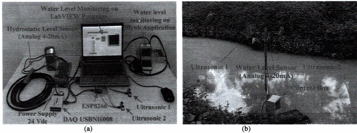
Fig. 8 Overall picture prototype of water level monitor and flood alarm (a) and testing installation (b).
