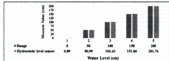
Fig. 9 The results of each water level reading of the measuring tool for displaying on the LabVIEW program with the measurement kit (Analog sensor 4 – 20mA).
