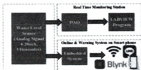
Fig. 2 The working diagram of a real-time prototype of water level monitor and wide area early flood warning.
