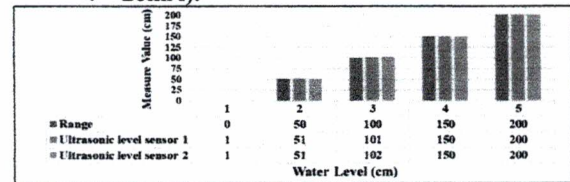
Fig. 10 The results of each water level reading of the measuring tool displayed on the Blynk application on a mobile phone with ultrasonic1 and ultrasonic2 measurement kits.
