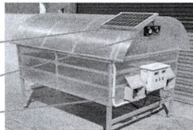
Fig. 3 Electric oven with solar energy
