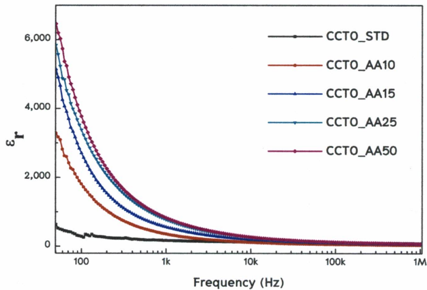
Figure 5 Dielectric constant values of CCTO with activated carbon derived from tamarind fruit shells.
