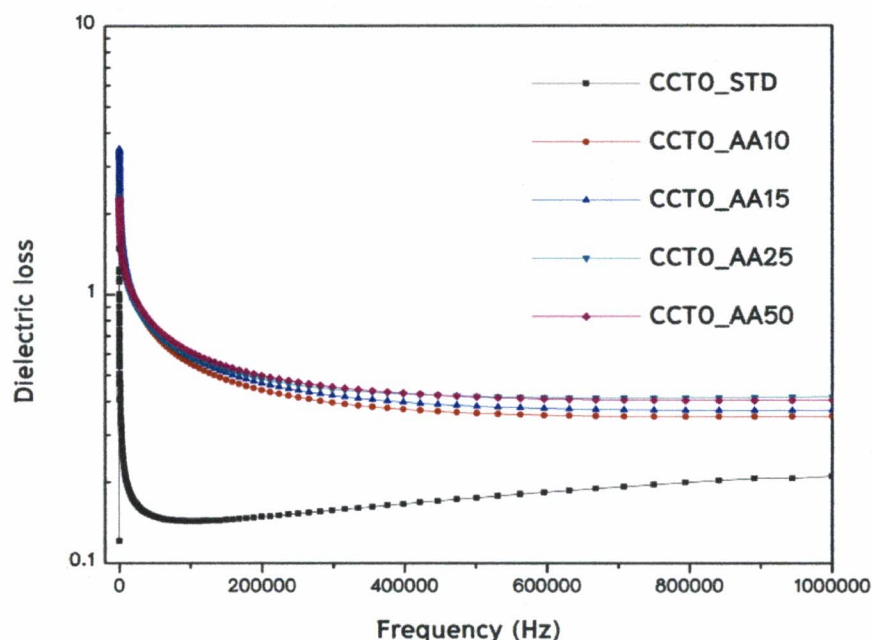
Figure 6 Dielectric loss of CCTO with activated carbon derived from tamarind fruit shells.
