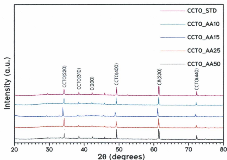
Figure 2 Phase patterns of CCTO with activated carbon derived from tamarind fruit shells.
