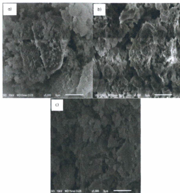
Figure 3 SEM images of activated carbon derived from tamarind fruit shells: a) BA-TPC, b) TPC-KOH and c) AA-TPC.
