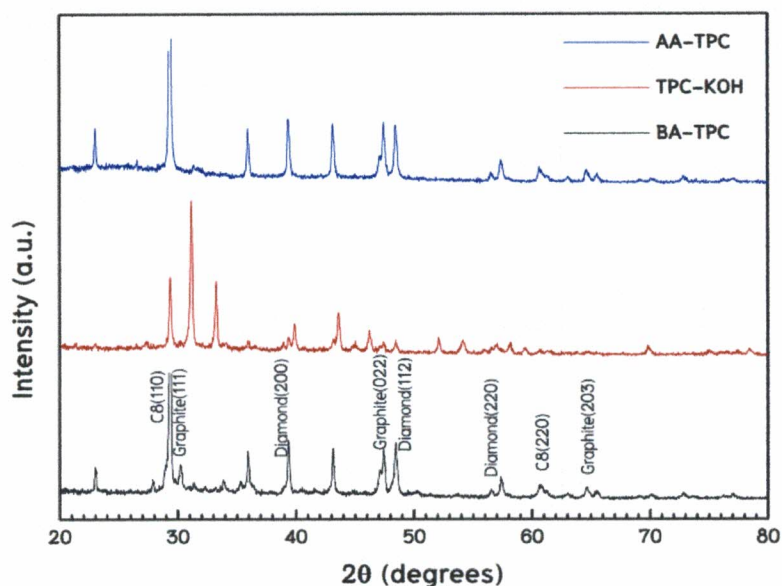
Figure 1 Phase patterns of activated carbon derived from tamarind fruit shells.
