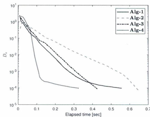
Figure 8. Numerical illustration of Algorithm 1 with Algorithm 1 in [28] and Algorithm 3.1 in [11] and Algorithm 3 in [31] for N=10 .
