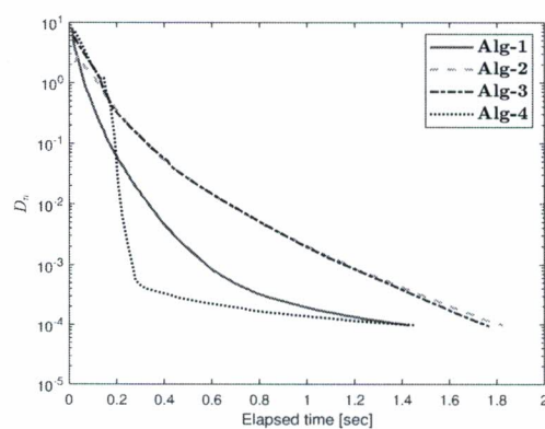
Figure 12. Numerical illustration of Algorithm 1 with Algorithm 1 in [28] and Algorithm 3.1 in [11] and Algorithm 3 in [31] for N=100 .
