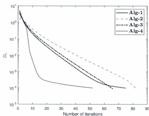
Figure 9. Numerical illustration of Algorithm 1 with Algorithm 1 in [28] and Algorithm 3.1 in [11] and Algorithm 3 in [31] for N=40 .
