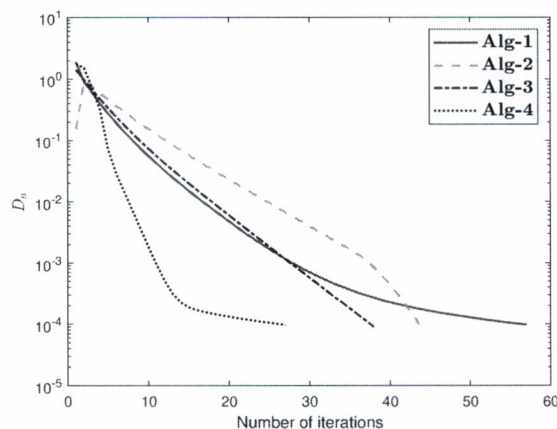
Figure 5. Numerical illustration of Algorithm 1 with Algorithm 1 in [28] and Algorithm 3.1 in [11] and Algorithm 3 in [31] for N=5 .
