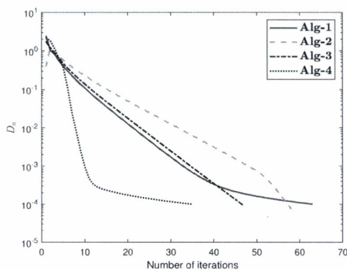
Figure 7. Numerical illustration of Algorithm 1 with Algorithm 1 in [28] and Algorithm 3.1 in [11] and Algorithm 3 in [31] for N=10 .
