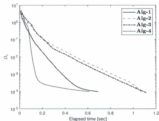
Figure 10. Numerical illustration of Algorithm 1 with Algorithm 1 in [28] and Algorithm 3.1 in [11] and Algorithm 3 in [31] for N=40 .
