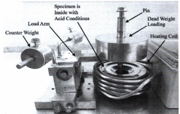
Figure 1 The Pin-on-Disc testing machine
