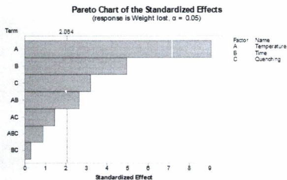
Figure 2 Pareto chart of the standardized effects.
