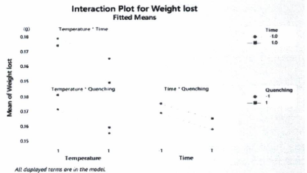
Figure 4 Interaction plot for weight lost
