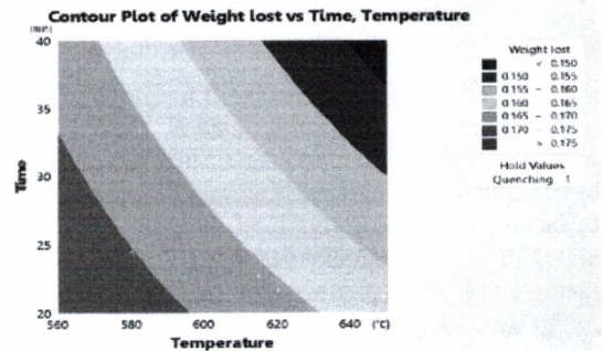
Figure 6 Contour plot of weight lost
