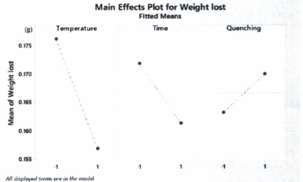
Figure 3 Main effects plot for weight lost
