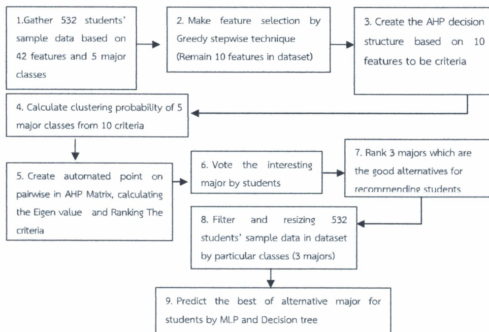
Figure 2 The algorithm of integrating the machine learning on AHP in students' decisions to study in universities
