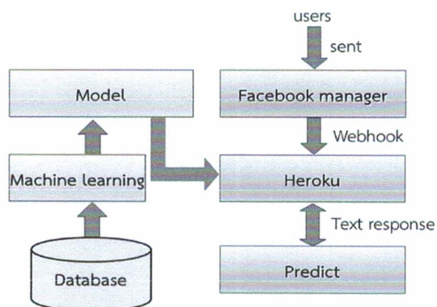
Figure 2 Framework of Messenger's Chatbot based on Artificial Intelligence for Digital Library Service
