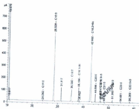
Fig. 1. GC chromatogram of coffee oil.
