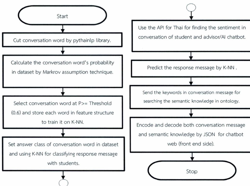
Figure 1 Flowchart of the artificial intelligence chatbot development
