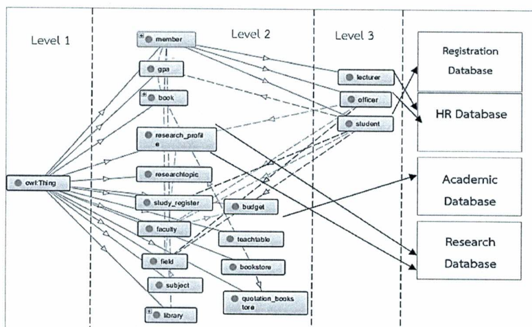
Figure 1 Library service knowledge base on topology and database fusion
